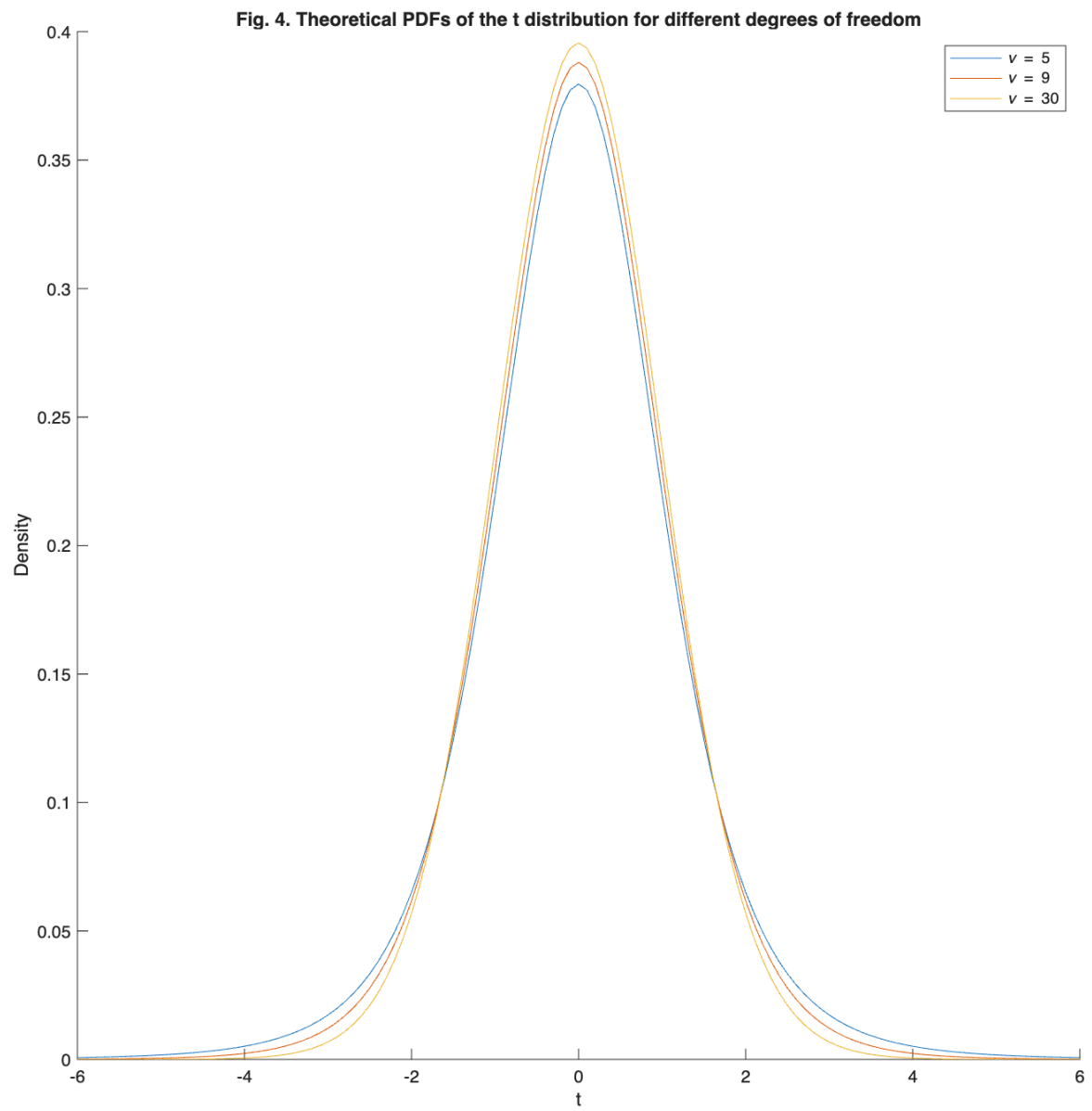
Figure 4: Limiting distributions with different degrees of freedom
